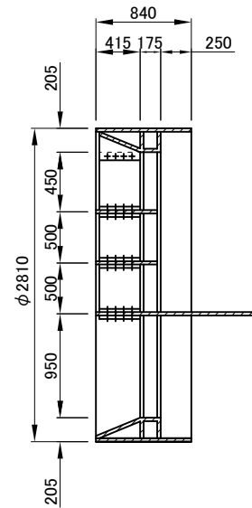
呼び径2400mm
